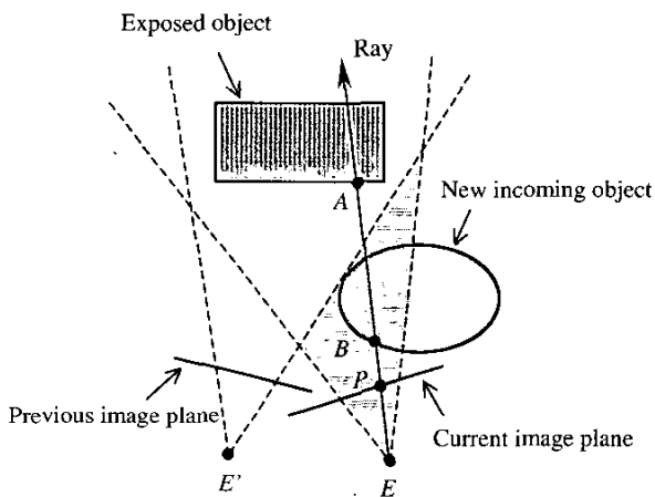
Figure 2. Emergence of new incoming objects.
