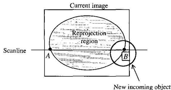
Figure 3. Detection of the new incoming objects.
