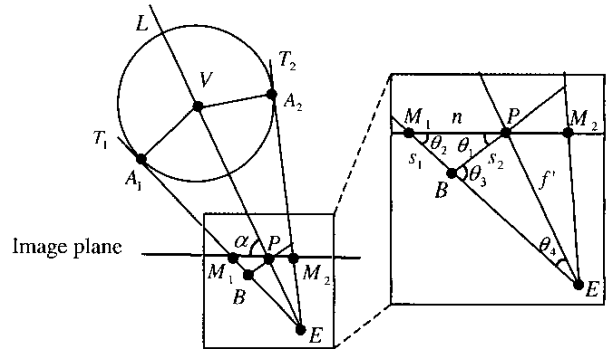
Figure 6. An example of bounding sphere projection.
