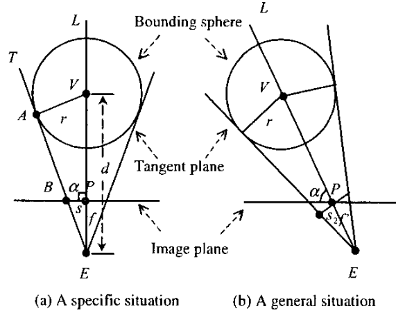
Figure 1. Bounding-sphere projection of a cell.
