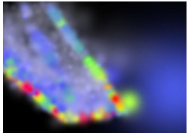
Figure 9: Resolution: r_3 .
