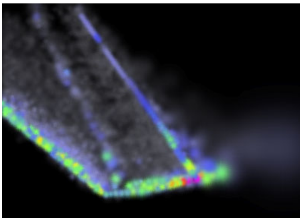
Figure 8: Resolution: r_2 .
