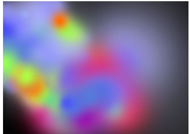
Figure 10: Resolution: r_4 .
