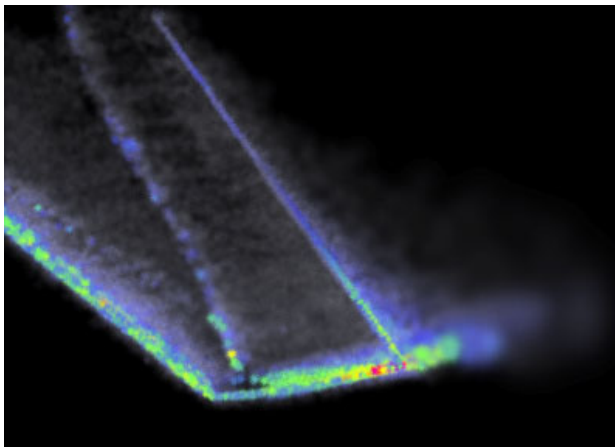
Figure 7: Resolution: r_1 .
