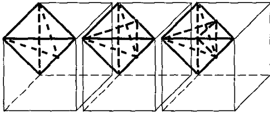
Figure 2: Three phases of refinement for a single tetrahedron of the initial configuration.
