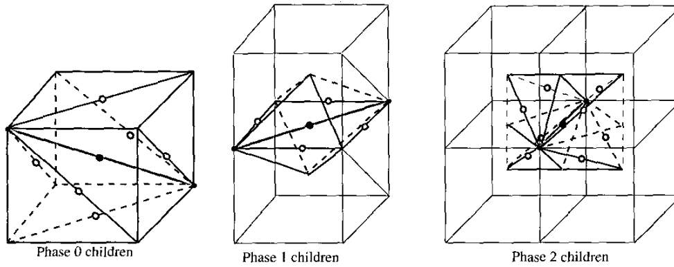
Figure 4: Child diamonds: Phase 0 children are located on the faces of a cube, phase 1 children are located on the centers of the edges of the face containing the split edge, and phase 2 children are the phase 0 diamonds from level L + 1 that touch the diamond's split edge.
