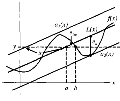
Figure 6: Isosurface error calculation in 1D.
