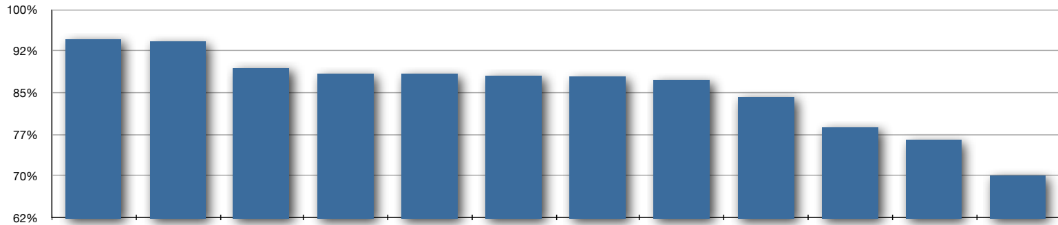
Current Scores
