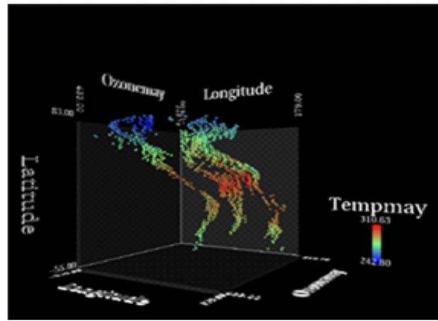
Figure 5(b): A 3D plot of Latitude (Y-axis), Longitude (X-axis), Ozone (Z-axis) and Temperature (color) on a TIC
