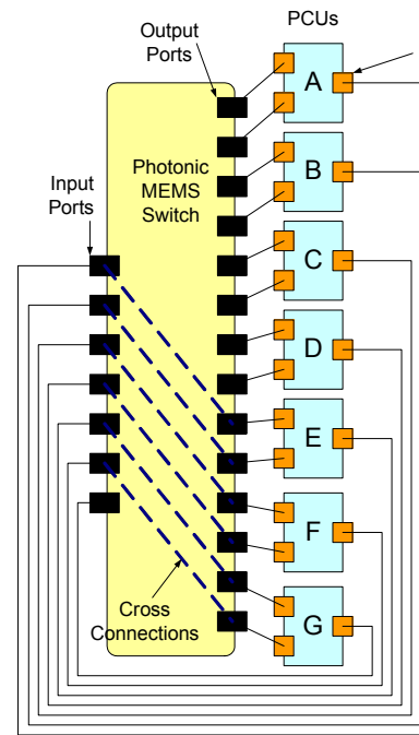
Figure 5: Creating the Sort-Last Rendering Engine using the Photonic Switch
