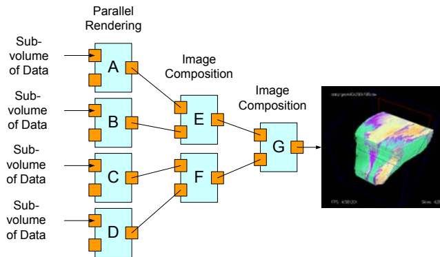
Figure 4: Photonic Computing Engine designed for Sort-Last Rendering
