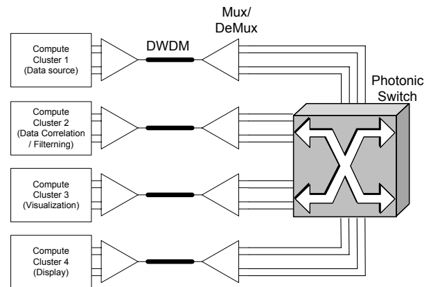
Figure 1: In the OptIPuter, a number of distributed compute clusters are interconnected via a photonic switch rather than with traditional routers. The optical transport platform performs the task of multiplexing and demultiplexing multiple light paths over a dense wave division multiplexed (DWDM), long haul network.
