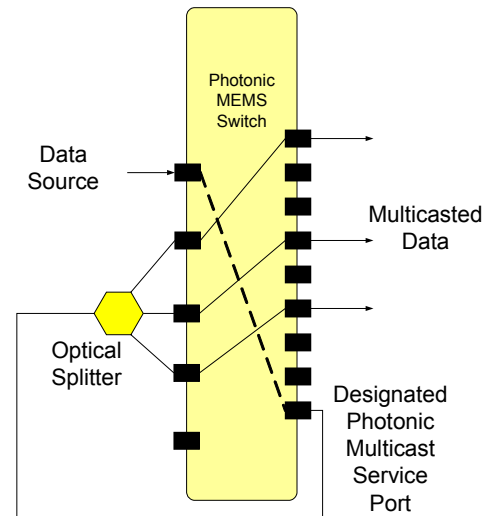
Figure 2: Schematic of how to integrate practical photonic multicasting in a photonic switch.
