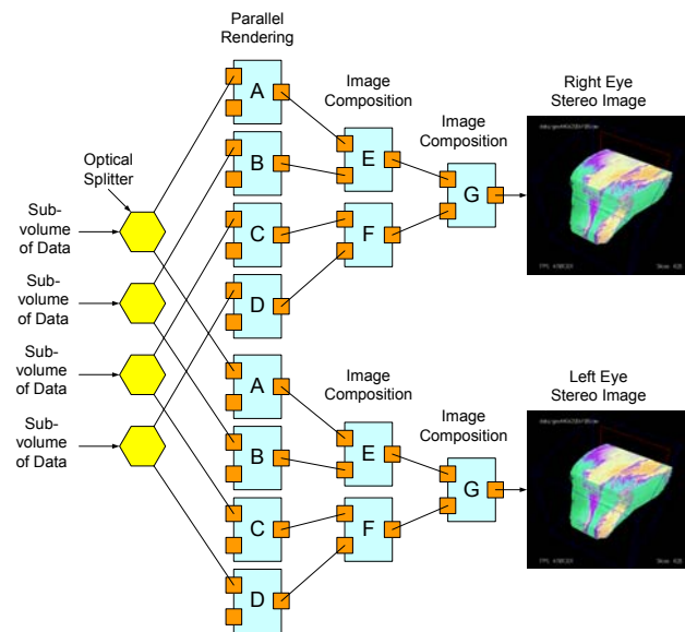
Figure 6: Taking advantage of photonic multicasting to mirror data to two Photonic Computing Engines.
