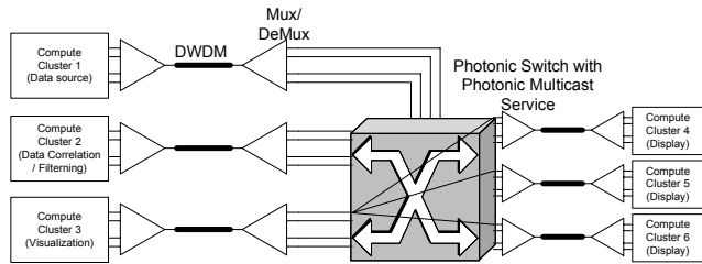
Figure 3: Integration of Photonic Multicasting into the Photonic Data Exploration Pipeline.
