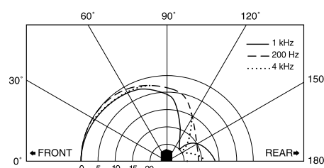
Fig. 2 Vertical Plane Polar Response
