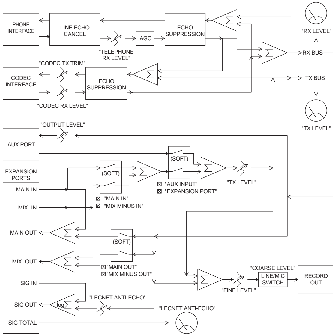
TH3 Block Diagram
