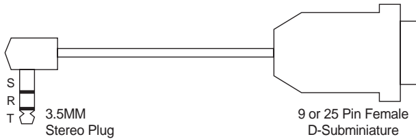
LecNet Device to PC
