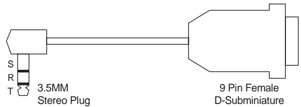
LecNet Device to AMX or Crestron
